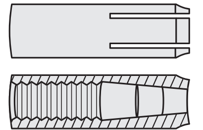
Drop-In Anchors
